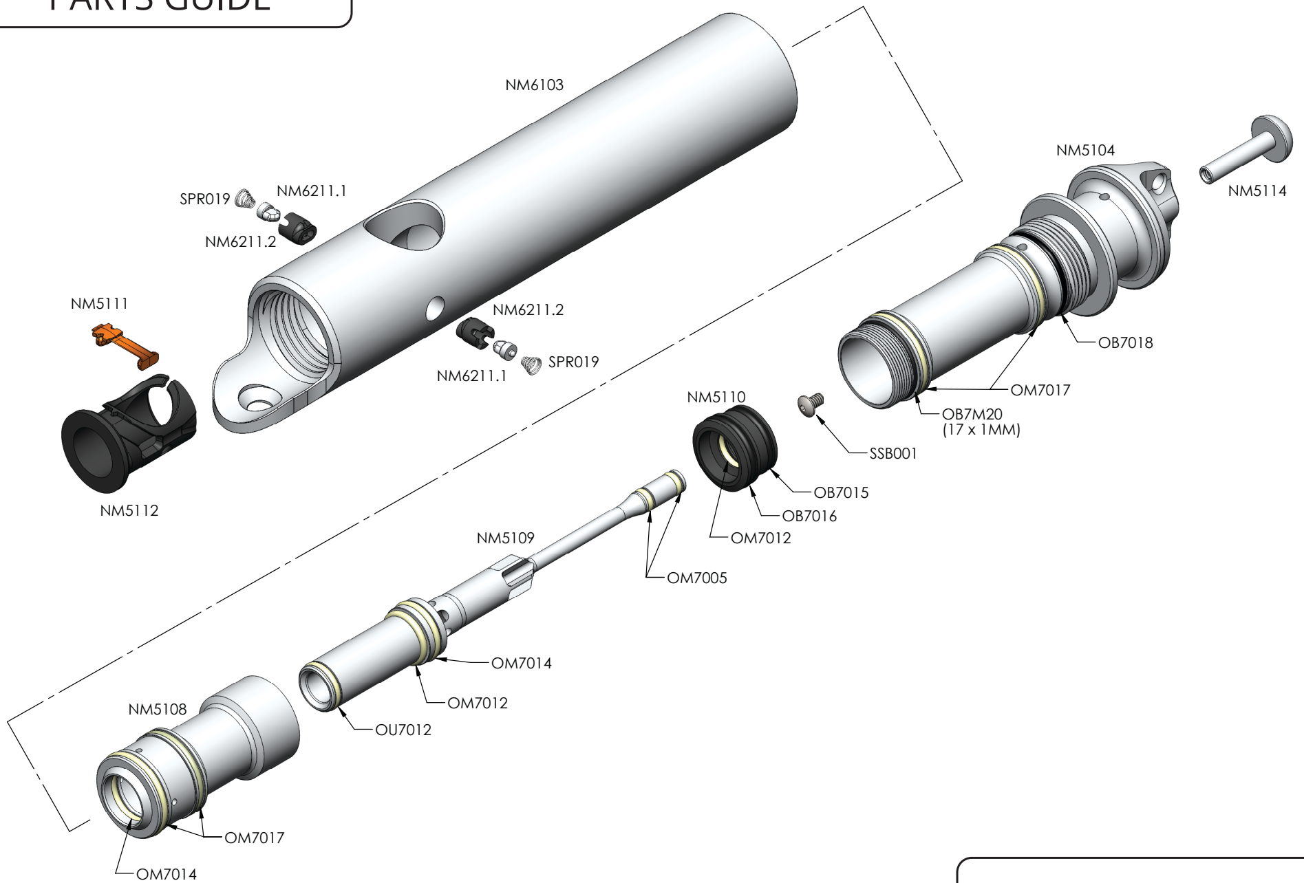
FIGURE 4 50 CAL. INTERNALS
